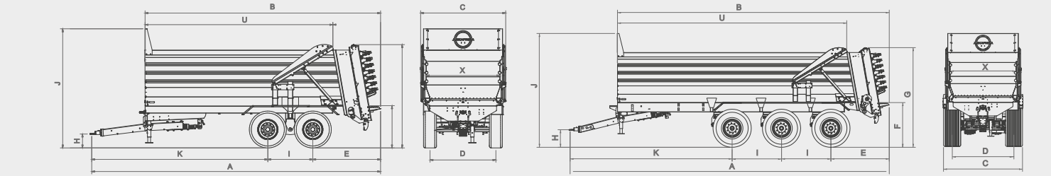
Available in models E95KMP2. Standard: Triple sidra self-steering axle in first and third axle, 2000 track, 10 bolts, brakes 400x120. Optional: Triple sidra forced steering axle in first and third axle commanded with cylinder attached to the tractor, 2000 track, 10 bolts, brakes 400x120. According to norm ISO 26402. Triple sidra forced steering axle in first and third axle commanded electronically, 2000 track, 10 bolts, brakes 400x120. Triple sidra forced steering axle in first, second and third axle commanded electronically, 2000 track, 10 bolts, brakes 400x120. Note: Include change from central axle to directional axle.
